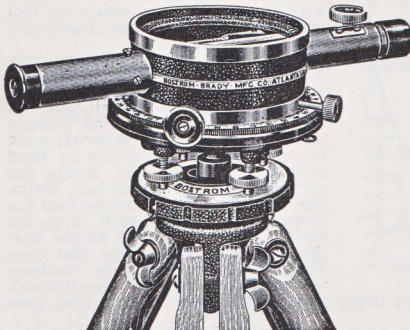
No. 4 CONTRACTOR'S LEVEL
